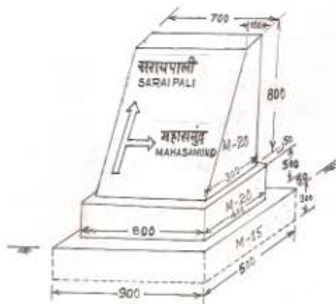
PERSPECTIVE VIEW
