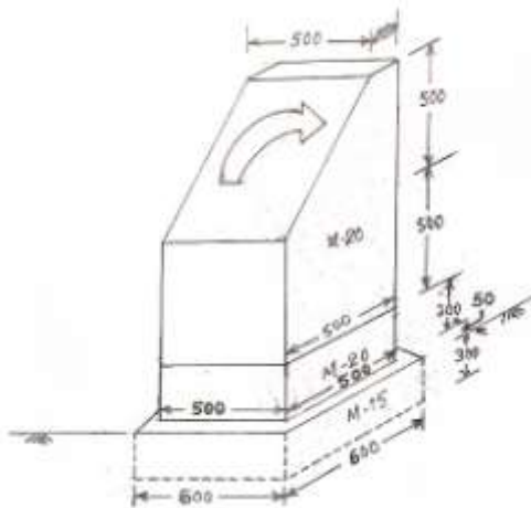
PERSPECTIVE VIEW
