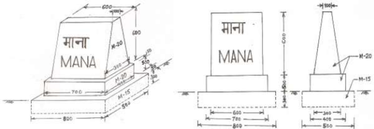
PERSPECTIVE VIEW
